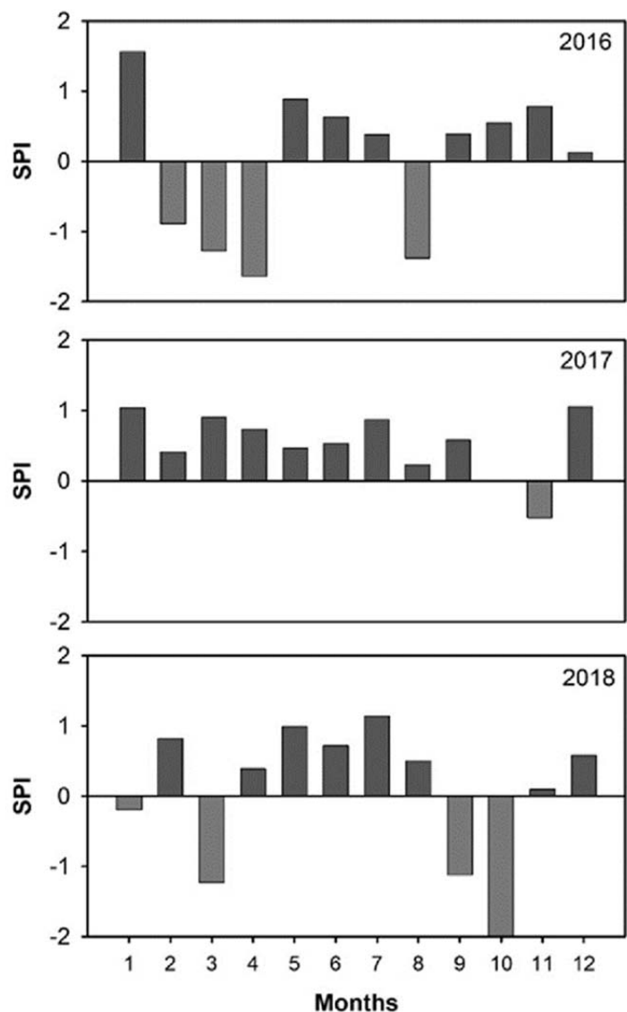
Suppl. Mat. Fig. 1 Standardized Precipitation Index (SPI) of the last three years for the experimental site at Wang Thong district, Phitsanulok province, Thailand. It was generated from 50 years of historical weather data at the location using National Drought Mitigation Center - SPI Generator 1.7.5.0. (Edwards & McKee, 1997).
