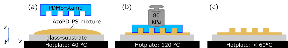
Figure 3. Schematic representation of structuring the AZOPD-PS film via tNIL. (a) 300 \mu L of an AZOPD-PS solution was dropcasted on a glass substrate and heated at 40 °C for 30 s to remove partly the solvent. (b) The PDMS stamp was placed onto the AZOPD-PS layer and a pressure of 80 kPa was applied for 30 min at 120 °C. (c) After cooling below 60 °C the PDMS stamp was separated.
