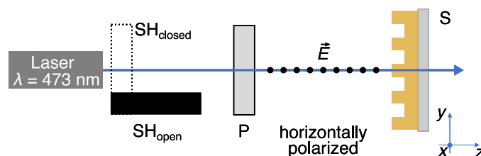
Figure 4. Schematic draw of the experimental setup. The linear polarization orientation \vec{E} along x -axis is ensured by a polarization filter P. The sample S was placed into a movable sample holder to align it in x - y -plane, which is perpendicular to the beam propagation ( z -axis). The automated shutter SH was placed in front of the laser to block the laser beam after the illumination duration.
