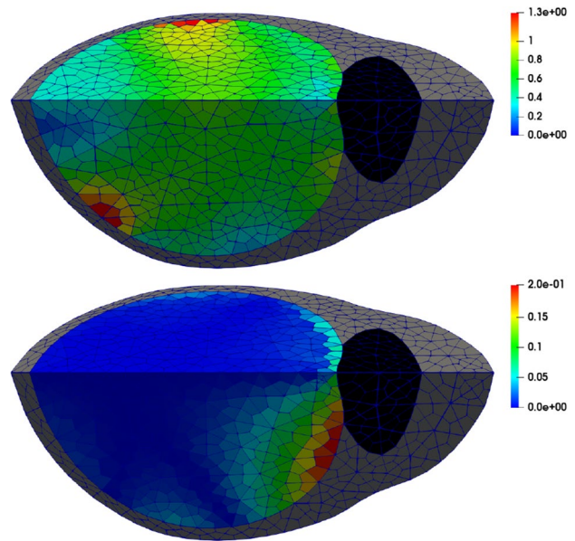
Fig. 12 Average norm per cell of the transformed Cauchy stress tensor J\hat{\mathbb{T}}_i\hat{\mathbb{F}}^{-T} in the vitreous for the Burgers (top) and the Navier–Stokes (bottom) case. The domain is cut vertically for visualization purposes
