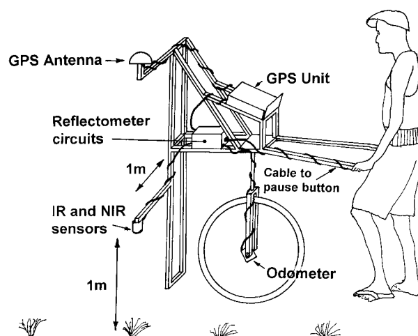
Fig. 1. Diagram of the radiometer operating in a pearl millet field showing its major components.
