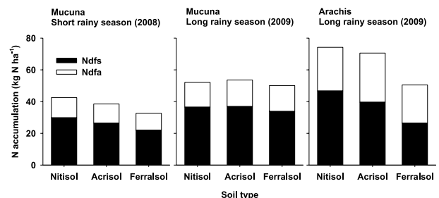
Fig. 2: Nitrogen accumulation of Mucuna pruriens var. utilis and Arachis pintoii (CIAT 18744) on three contrasting soil types in Kakamega, Kenya. Bars are standard error of means ( n = 4 ). Mucuna pruriens was evaluated at 6 weeks after seeding in the short rainy season (2008) and the long rainy season (2009). Arachis pintoii was evaluated after 12 months at the end of the long rainy season (2009).
