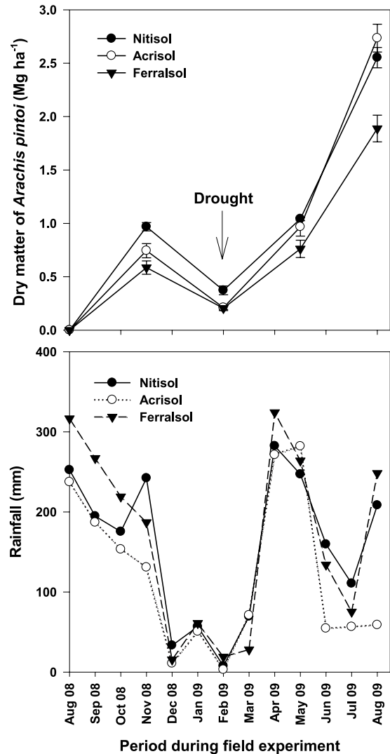
Fig. 1: Sequential dry matter of Arachis pintoii (CIAT 18744) and rainfall distribution with time after seeding between August 2008 and August 2009 on three contrasting soil types in Kakamega, Kenya. Bars are standard error of means ( n = 4 ).
