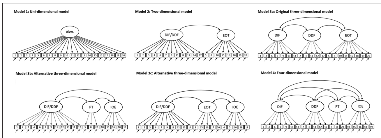
Figure 1. Competing measurement models for the TAS-20.
