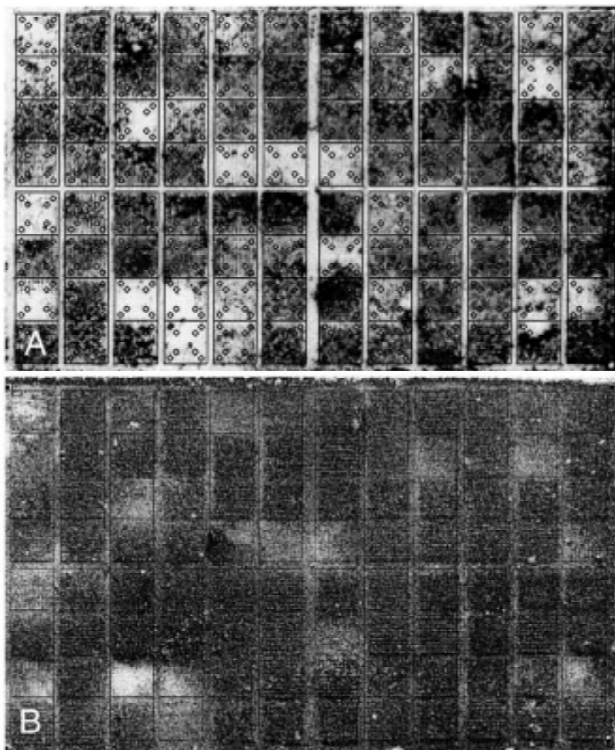
Figure 1. Normalised green band image with destructive sampling areas (the darker the pixels the denser the vegetation) derived from the aerial photograph taken at peak fallow vegetation on 18 August 1998 (A) and normalised red band from the aerial photograph taken on 18 June 1997 showing soil reflectance differences (crusted areas appear lighter) between mulched and unmulched plots (B). The experiment measured 140 \times 83 m, size of individual plots was 10 \times 10 m.
