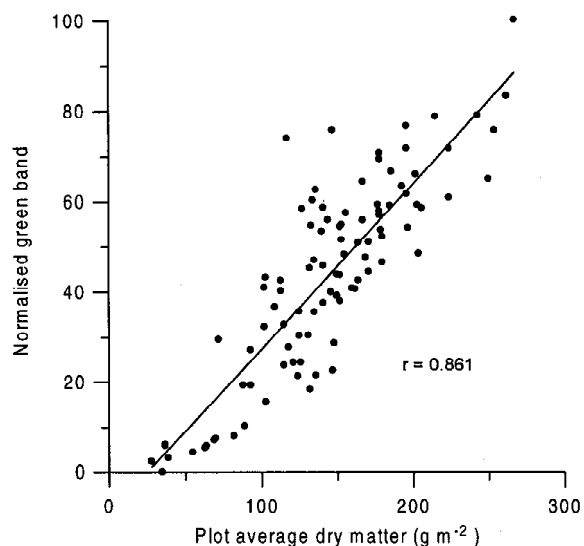
Figure 3. Relationship between normalised green band of the 18 August 1998 aerial photograph and destructively determined herbaceous dry matter (HDM) measured on 26 August 1998. Data points show averages of eight replications at the plot level.
