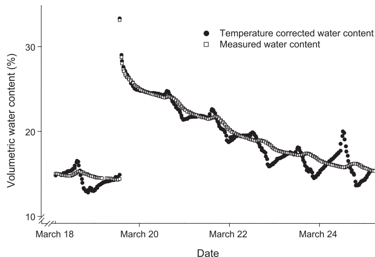
Fig. 3. Soil water dynamics during 7 days in an alfalfa-planted field at the mountain oasis Balad Seet (Oman) in March 2002 with and without the temperature correction for the volumetric water content ( \theta ) as provided by the probe manufacturer.
