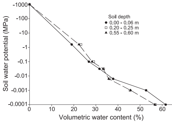
Fig. 6. Soil water characteristic function showing water contents at different soil water potentials for three depths of a terrace soil at the mountain oasis of Balad Seet, Oman. Vertical bars indicate \pm one standard error.
