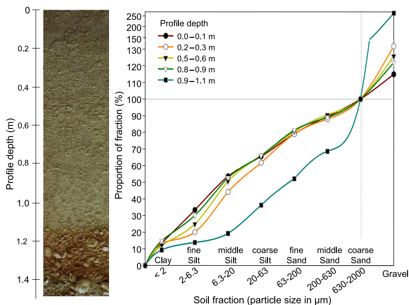
Fig. 2. Soil profile of the lower part of the Mazra terrace system at the mountain oasis Balad Seet (Oman) planted with annual crops and alfalfa. Note the difference between the gray, silt-rich upper layers of this man-made profile with their high water-holding capacity and the lower portion with its reddish, stony and rapidly draining structure (left) and the large difference in the particle size distribution curve below 0.9 m (right). The value of 100% refers to the mass of the mineral soil, the gravel fraction is not included in the mineral soil and thus leads to numbers exceeding 100%.
