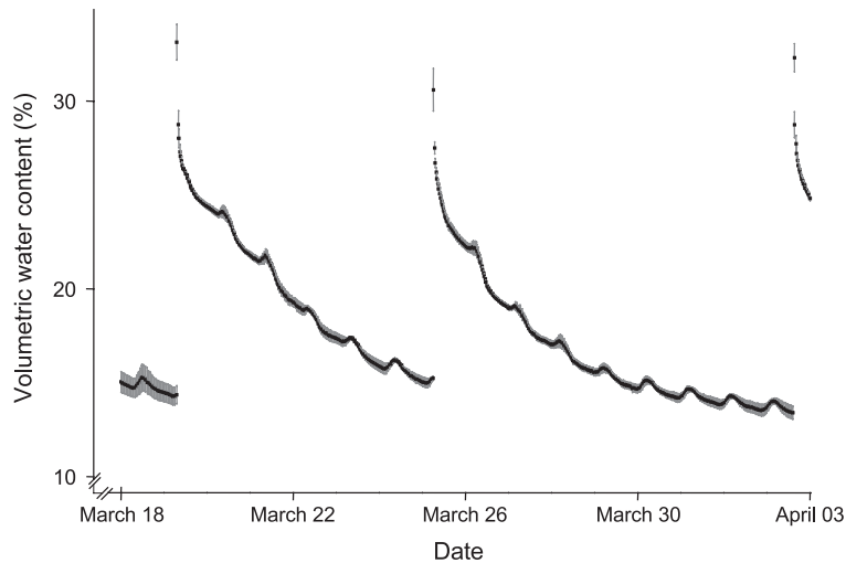
Fig. 4. Soil water dynamics during two irrigation cycles in an alfalfa-planted field at the mountain oasis Balad Seet (Oman) in March and April 2002. The data are means of four probes with the grey bars indicating \pm one standard error.
