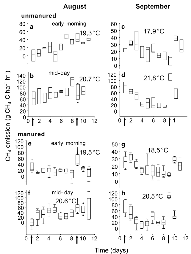
Fig. 5: Time course of CH 4 emissions from plots without and with manure application in the mountain oasis of Al' Ayn (Oman) in August and September 2006. Irrigation occurred at day 1 and 9 as indicated by the arrows. Average soil temperatures are indicated. The boxplots show the median, the 10th, 25th, 75th and 90th percentiles as well as the outliers of five measured gas concentrations at sample integration times of 5 s for CO 2 and NH 3 , 20 s for CH 4 , and 50 s for N 2 O. The boxplot-like figures in the unmanured treatments show the three measured values.
