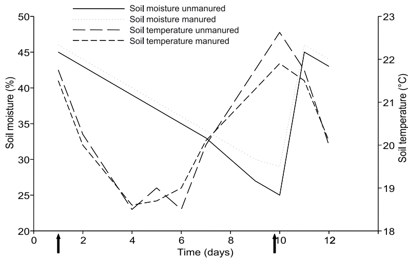
Fig. 3: Time course of average soil moisture and temperature of manured and unmanured plots without tillage in Al' Ayn (Oman) in August 2006. Irrigation occurred on day 1 and 10 as indicated by the arrows.
