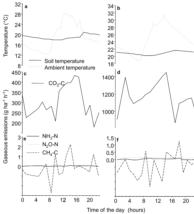
Fig. 2: Day course of soil and ambient temperature and gaseous emissions in fodder wheat from an untilled plot in mountain oases of Al Qasha' and a tilled plot in Al' Ayn (Oman), both under pomegranate in March 2006.
