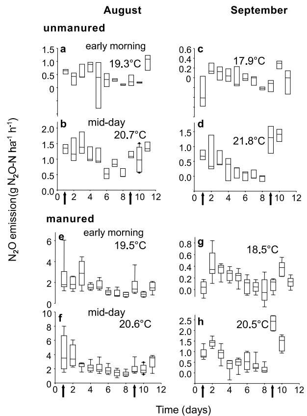
Fig. 7: Time course of \text{N}_2\text{O} emissions from plots without and with manure application in the mountain oasis of Al' Ayn (Oman) in August and September 2006. Irrigation occurred at day 1 and 9 as indicated by the arrows. Average soil temperatures are indicated. The boxplots show the median as well as the 10th, 25th, 75th and 90th percentiles. The boxplots show the median, the 10th, 25th, 75th and 90th percentiles as well as the outliers of five measured gas concentrations at sample integration times of 5 s for \text{CO}_2 and \text{NH}_3 , 20 s for \text{CH}_4 , and 50 s for \text{N}_2\text{O} . The boxplot-like figures in the unmanured treatments show the three measured values.
