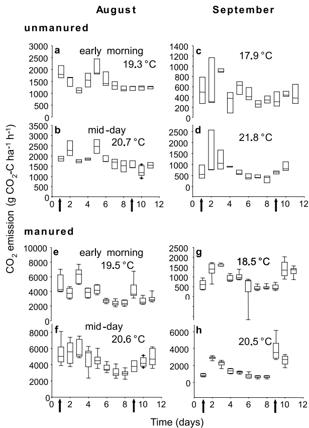
Fig. 4: Time course of CO 2 emissions from plots without and with manure application in the mountain oasis of Al' Ayn (Oman) in August and September 2006. Irrigation occurred at day 1 and 9 as indicated by the arrows. Average soil temperatures are indicated. The boxplots show the median, the 10th, 25th, 75th and 90th percentiles as well as the outliers of five measured gas concentrations at sample integration times of 5 s for CO 2 and NH 3 , 20 s for CH 4 , and 50 s for N 2 O. The boxplot-like figures (a-d) in the unmanured treatments show the three measured values.
