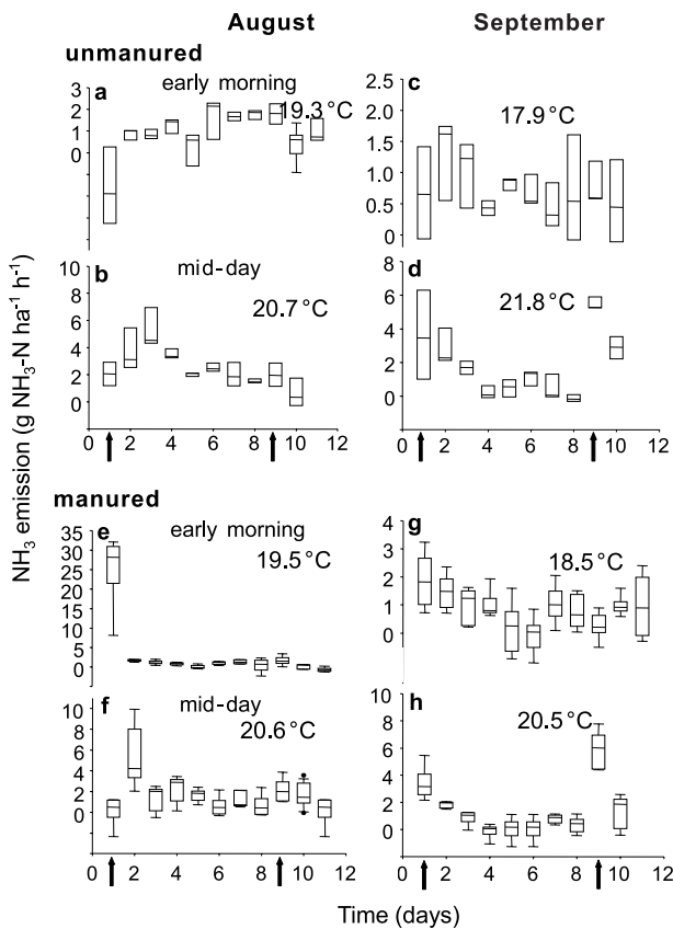
Fig. 6: Time course of \text{NH}_3 emissions from plots without and with manure application in the mountain oasis of Al' Ayn (Oman) in August and September 2006. Irrigation occurred at day 1 and 9 as indicated by the arrows. Average soil temperatures are indicated. The boxplots show the median, the 10th, 25th, 75th and 90th percentiles as well as the outliers of five measured gas concentrations at sample integration times of 5 s for \text{CO}_2 and \text{NH}_3 , 20 s for \text{CH}_4 , and 50 s for \text{N}_2\text{O} . The boxplot-like figures in the unmanured treatments show the three measured values.
