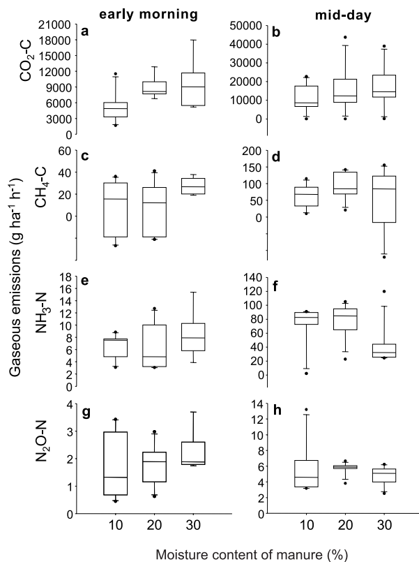
Fig. 1: Gaseous emissions from manure in a closed PE-fibre bag in the mountain oasis of Al' Ayn (Oman) in August 2006. Measurements were measured on the top of the bag. The boxplots show the median, the 10th, 25th, 75th and 90th percentiles as well as the outliers of 10 measured gas concentrations at sample integration times of 5 s for \text{CO}_2 and \text{NH}_3 , 20 s for \text{CH}_4 , and 50 s for \text{N}_2\text{O} .
