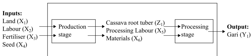
Fig. 1: The cassava production system.
